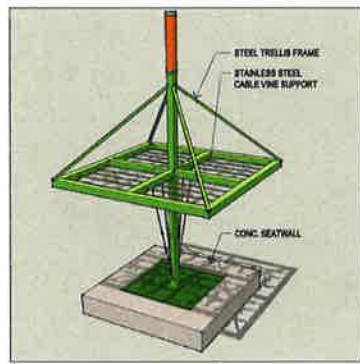
MAJOR PEDESTRIAN NODE SEATWALL W/ TRELLIS
