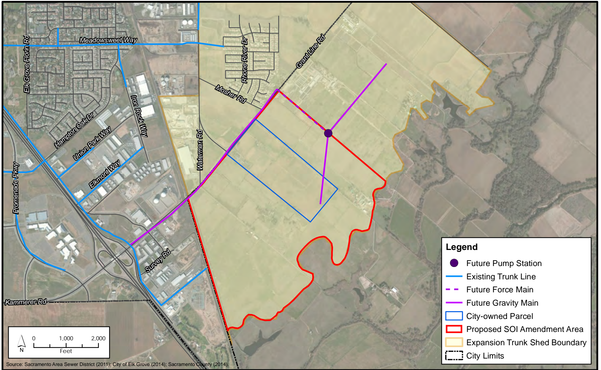
Figure 4.2-2 Sacramento Area Sewer District Master Plan for the LA Elk Grove Trunk Shed
