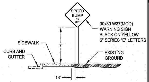
W37(MOD) ADVANCE SIGNING NOT TO SCALE
