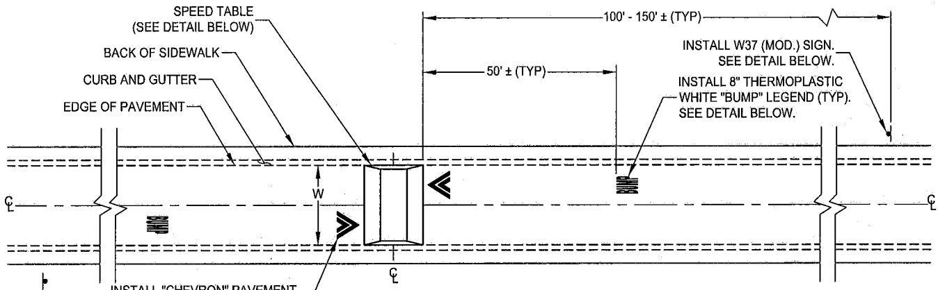
SIGNING AND STRIPING DETAIL NOT TO SCALE
