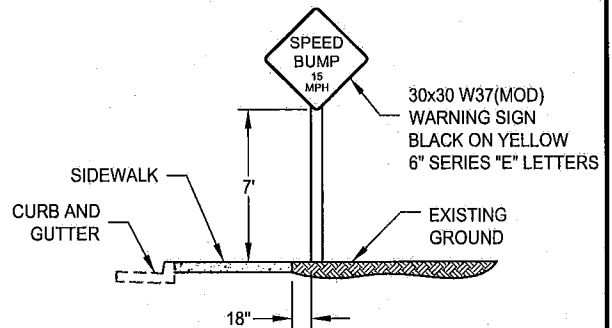
W37(MOD) ADVANCE SIGNING NOT TO SCALE
