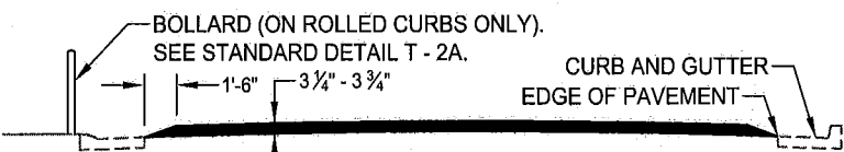
SECTION B-B NOT TO SCALE
