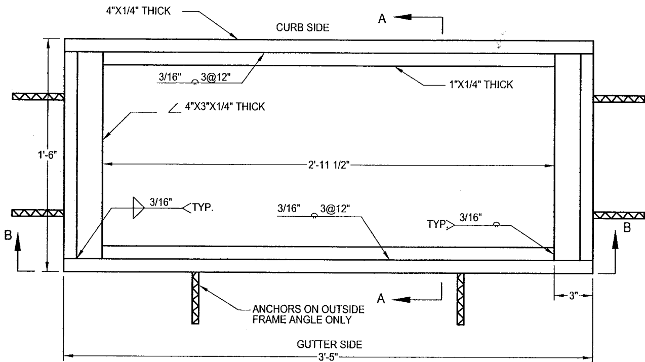
PLAN
