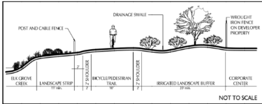
LAGUNA SPRINGS CORPORATE CENTER MASTER PLAN - TRAIL SECTION
